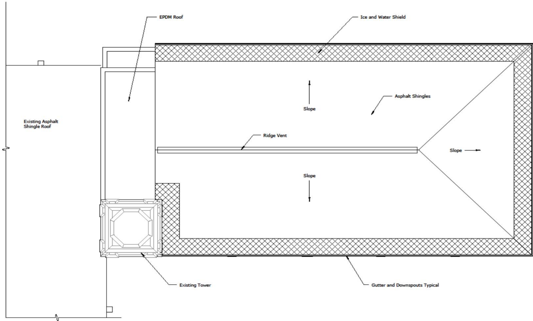
A14 Roof Plan 1/8" = 1'-0"
