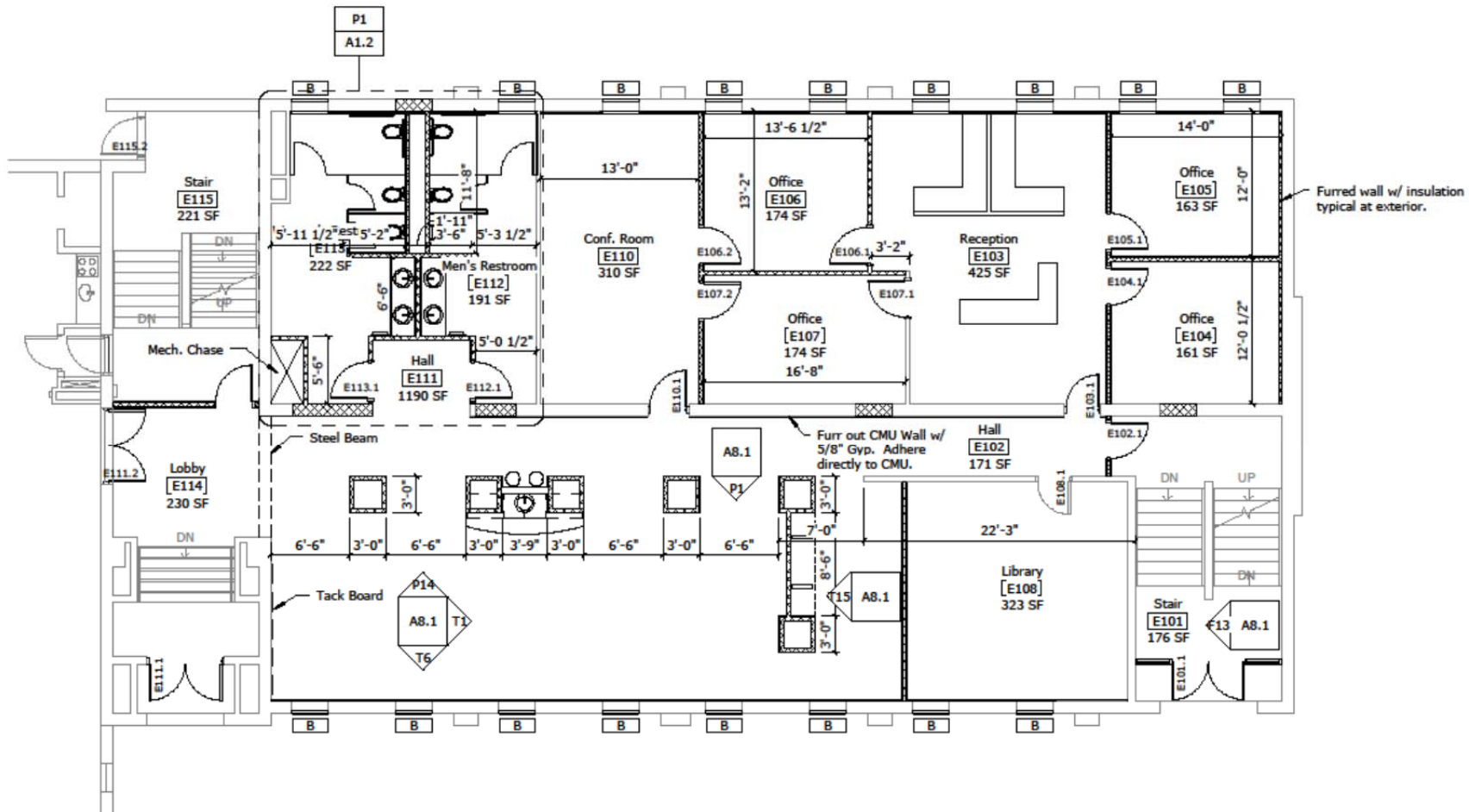
K1 First Floor Plan 1/8" = 1'-0"
